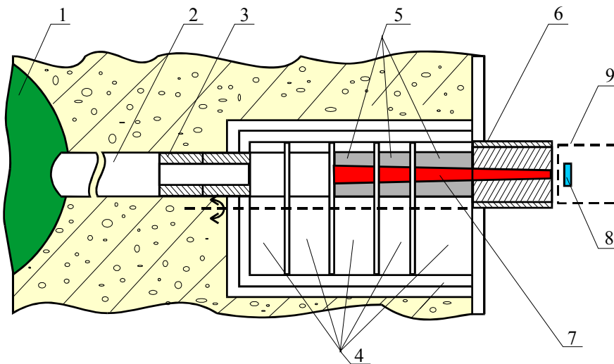
Fig. 2. Construction of forming system of filtered neutron beam on the KRR to obtain the quasi-mono-energetic neutron line. 1 – beryllium reflector; 2 – horizontal channel tube; 3 – preliminary collimator; 4 – beam shutter disks; 5 – filter-collimator assemblies; 6 – outside collimator; 7 – filter components; 8 – sample for activation; 9 – device for samples removing.
