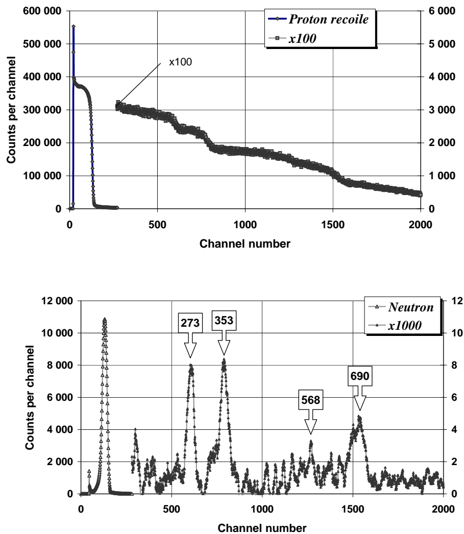
Fig. 3. Instrumental spectrum from proton recoil counter after neutron filter with energy 59 keV (top picture), and the shape of neutron filtered beam spectrum obtained by differentiation of previous curve (lower picture).
