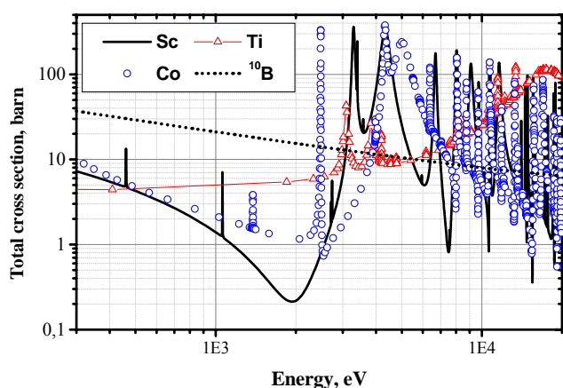
Fig. 1. Total neutron cross sections for Sc, Ti, Co, and ^{10}\text{B} in the energy range from 0.3 to 20 keV (JENDL-3.3 library).
