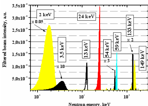
Fig. 4. Neutron filters used in the NPD for fundamental investigation.
